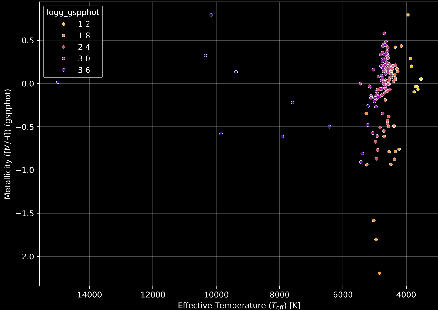
APOGEE DR17 Field: [M54SGRC-2] Stellar Population Parameters (n= 159)
