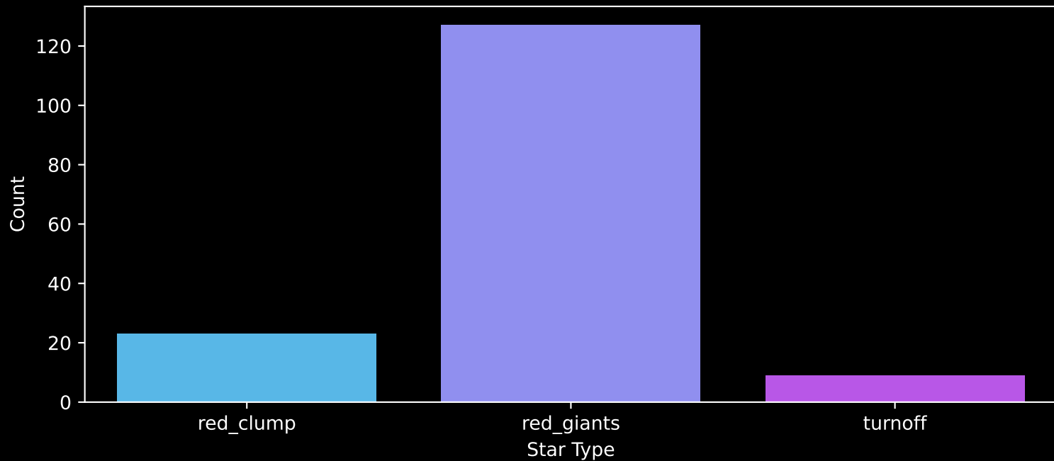
APOGEE DR17 Field: [M54SGRC-2] Count plot of Star Type
