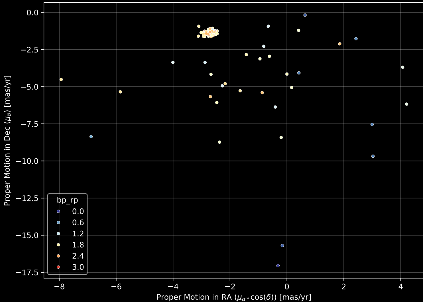
APOGEE DR17 Field: [M54SGRC-2] Proper Motion Diagram (n= 159)
