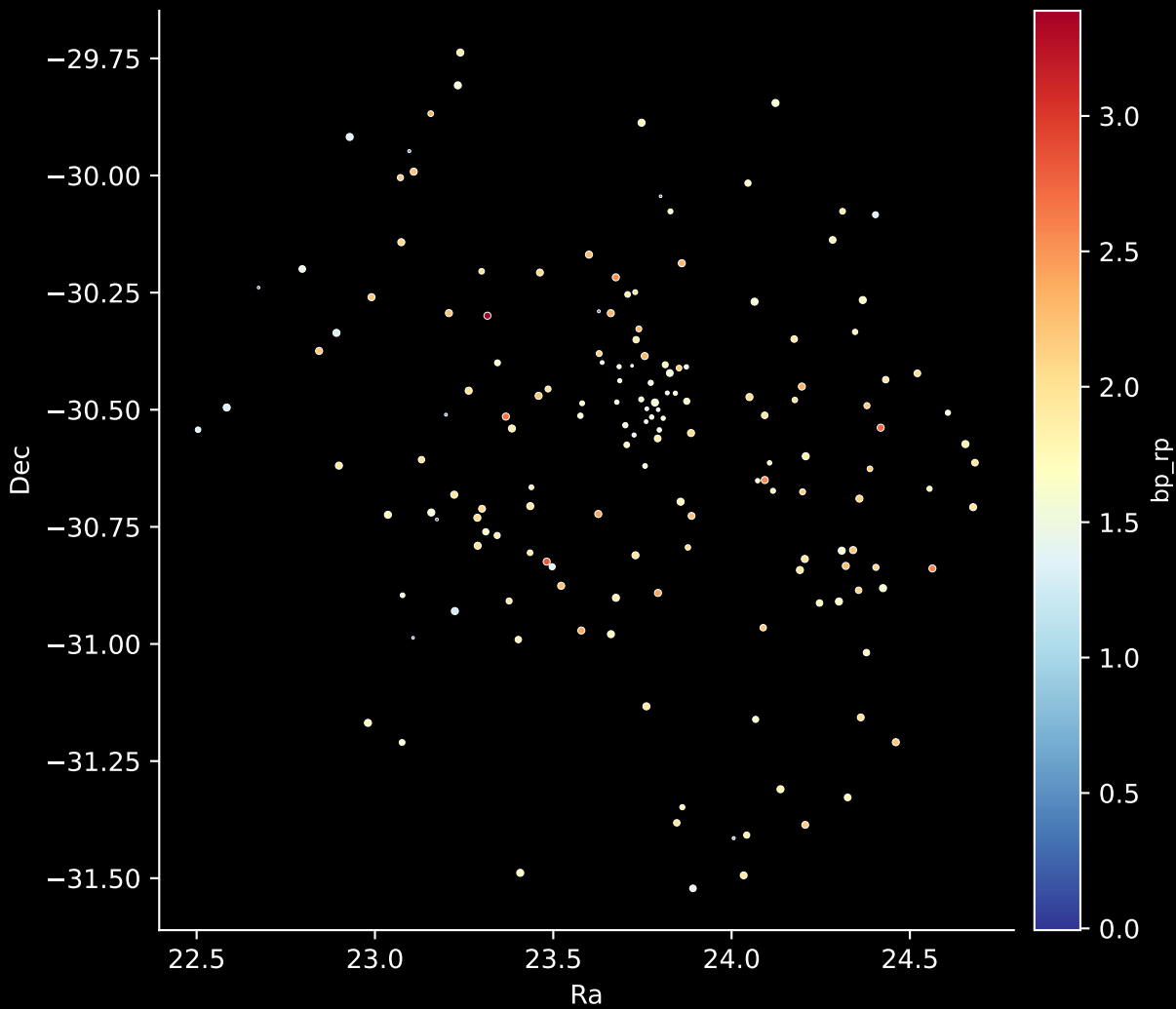
APOGEE DR17 Field: [M54SGRC-2] Stars: 159
