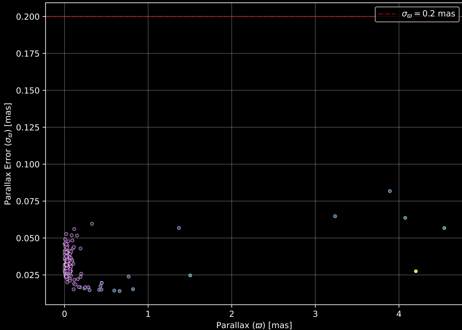
APOGEE DR17 Field: [M54SGRC-2] Parallax Quality (n= 159)
