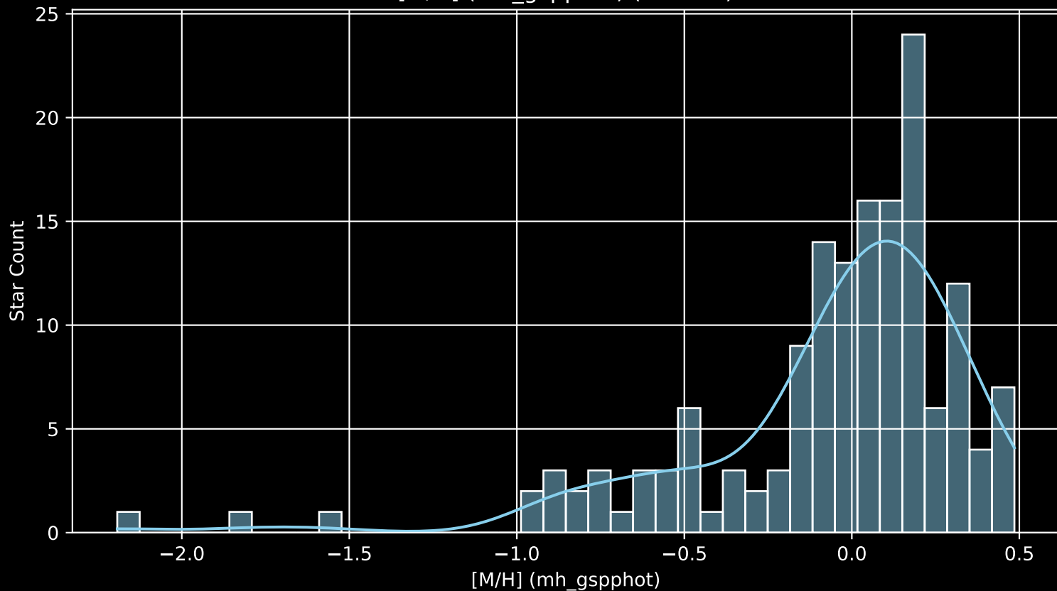
APOGEE DR17 Field: [M54SGRC-2 [M/H] (mh_gspphot) (n= 156)
