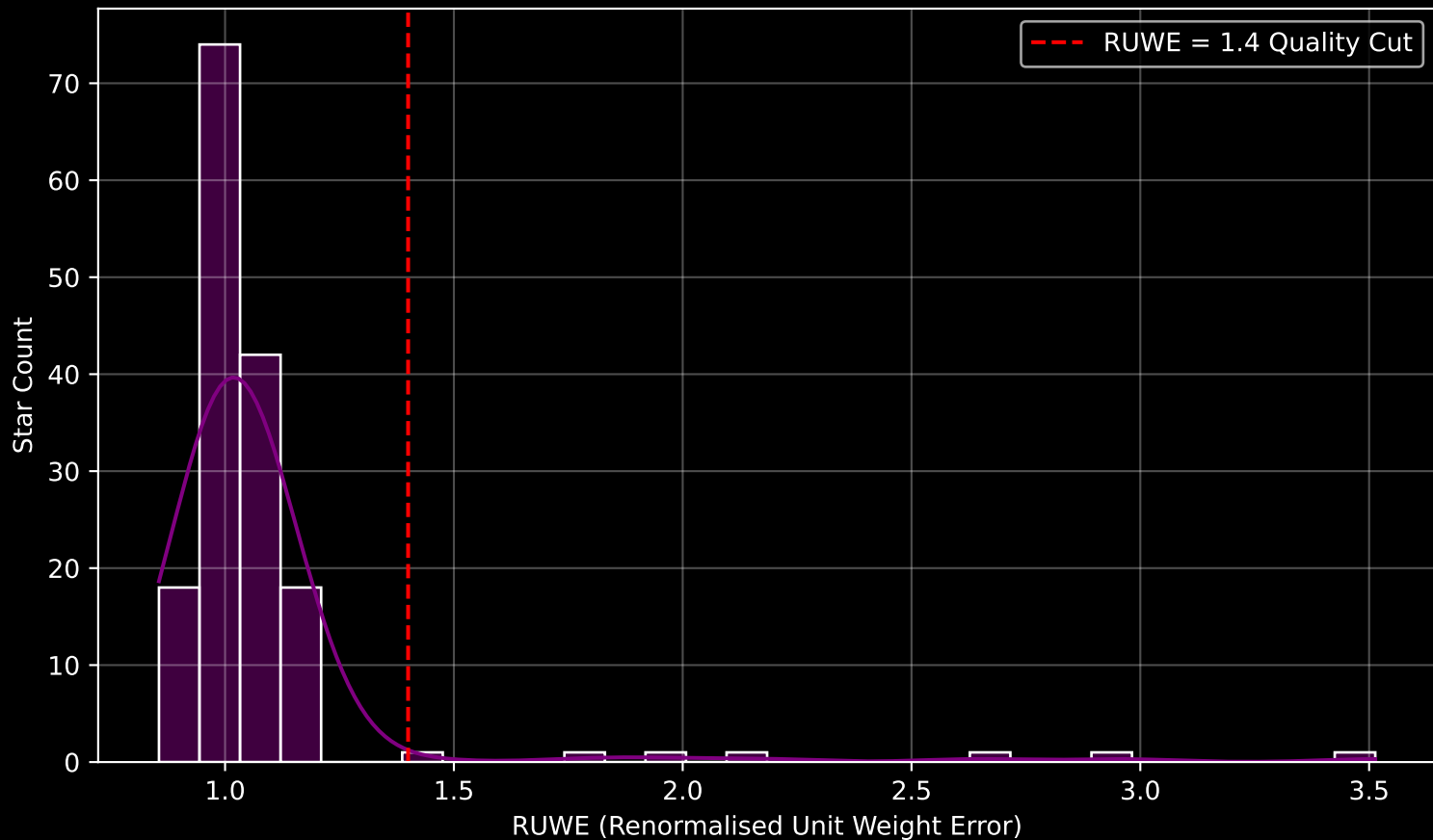
GAPOGEE DR17 Field [M54SGRC-2] RUWE Distribution (n= 159)
